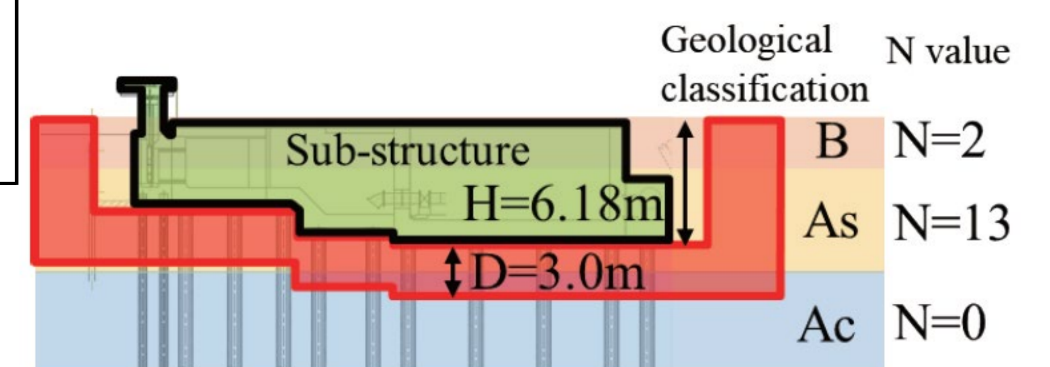
(b)Cross-section
