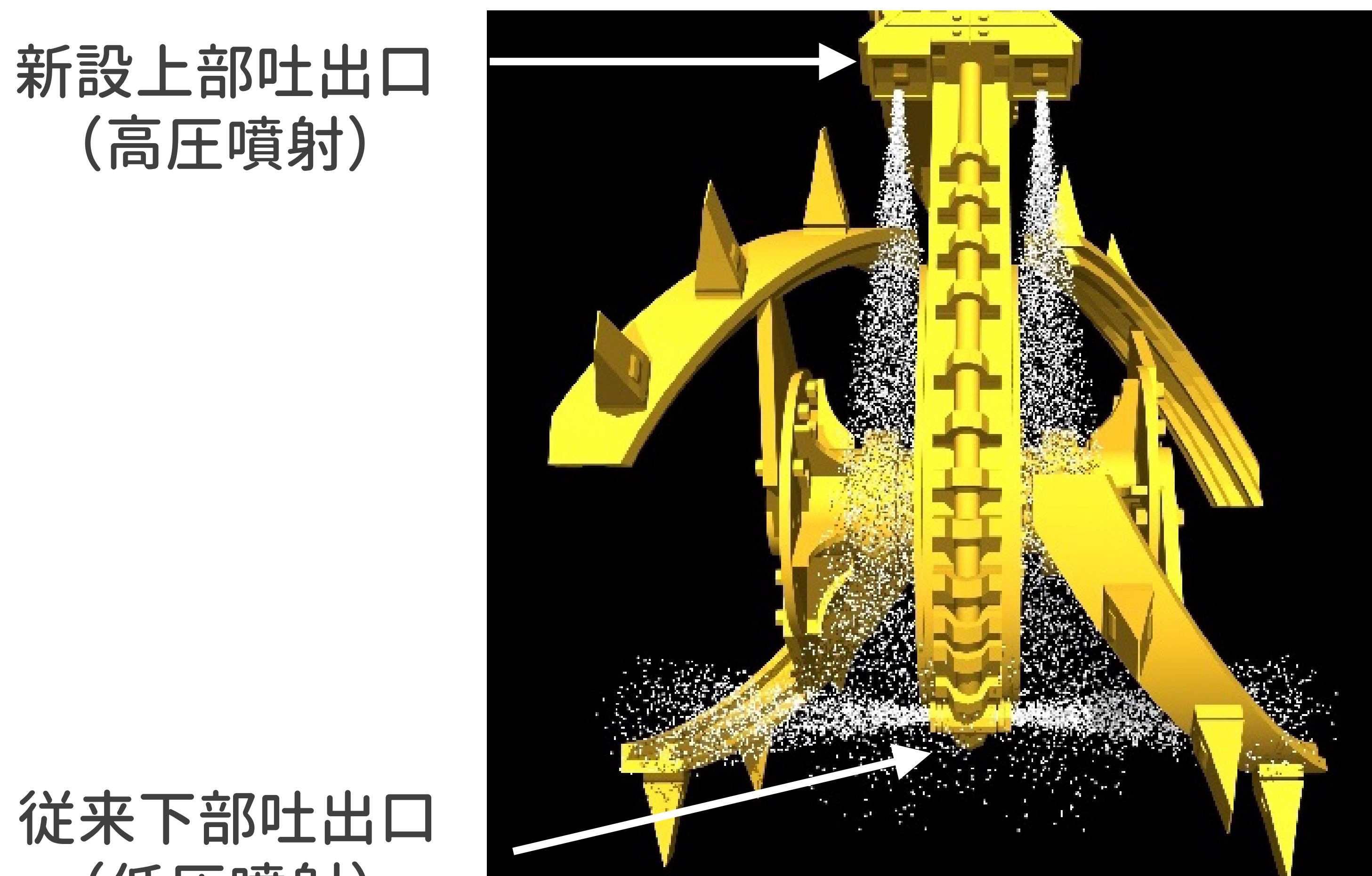
WILL-m工法攪拌翼
